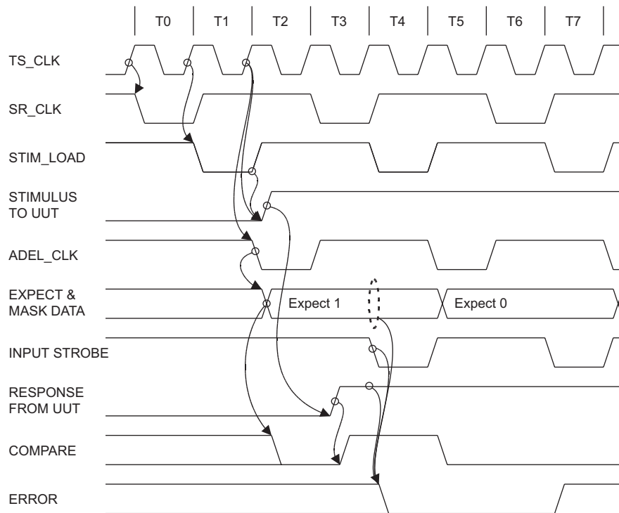
Figure 4-21 Input Mode 4 Timing
