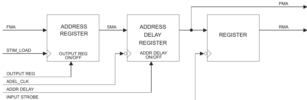
Figure 4-11 Input Address Logic Block Diagram
