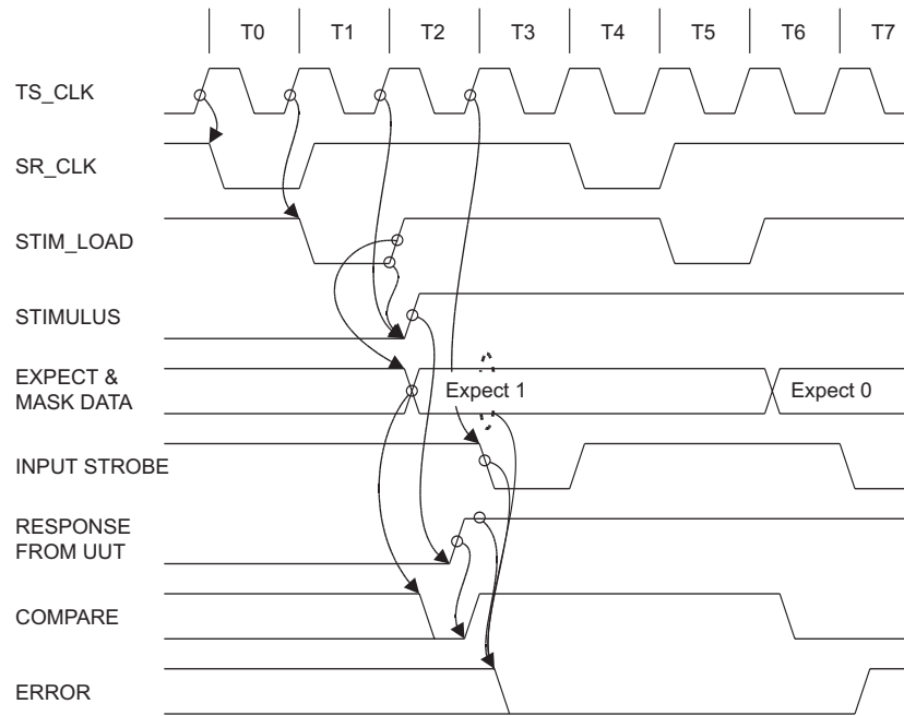
Figure 4-16 Input Mode 1 Timing
