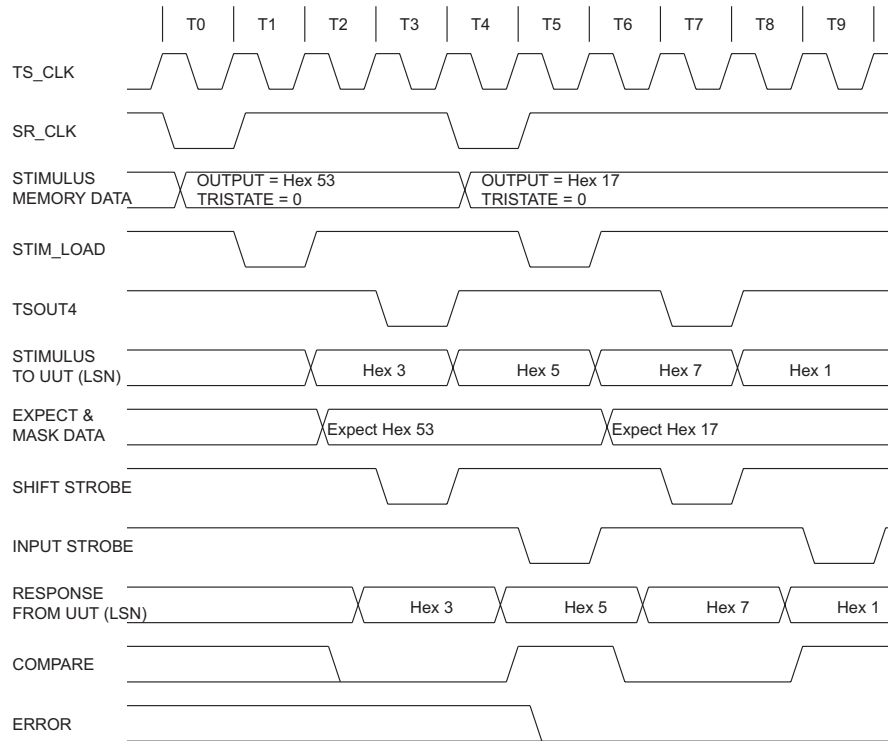
Figure 4-24 Multiplex Timing Example
