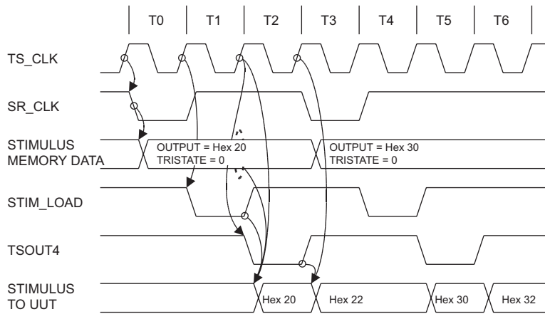
Figure 4-5 INCREMENT2 Timing Example
