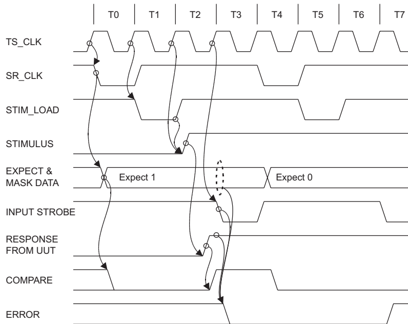
Figure 4-20 Input Mode 3 Timing
