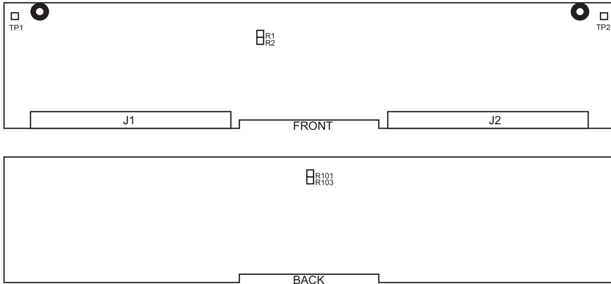
Figure 3-1 Test Point/Jumper Locations
