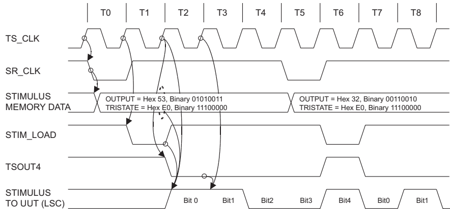
Figure 4-8 Serial Shift Timing
