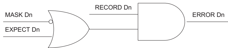
Figure 4-13 Error Memory Logic
