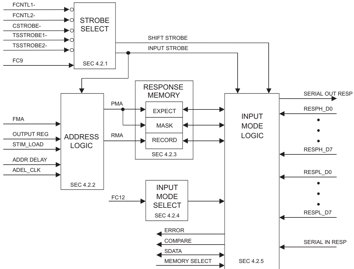
Figure 4-10 Response Logic Block Diagram
