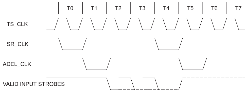
Figure 4-22 Input Mode 4 Timing Restrictions
