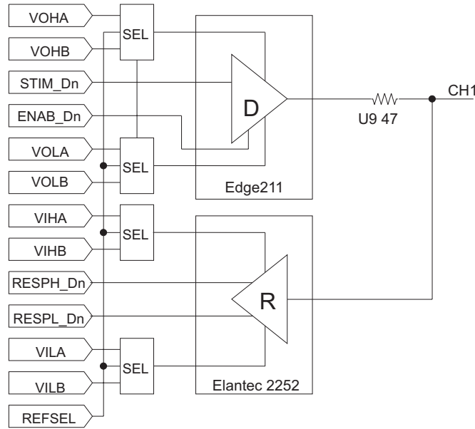
Figure 4-25 Driver/Receiver Logic Block Diagram
