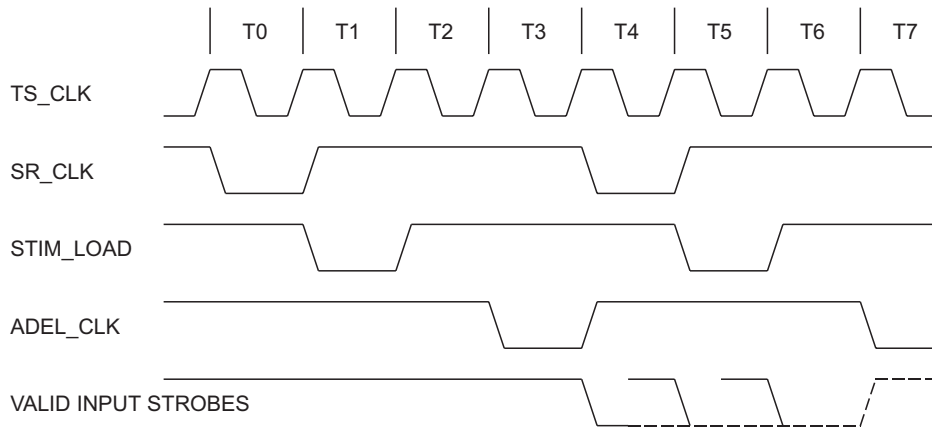
Figure 4-18 Input Mode 2 Timing Restrictions
