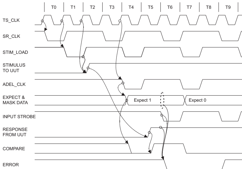
Figure 4-17 Input Mode 2 Timing
