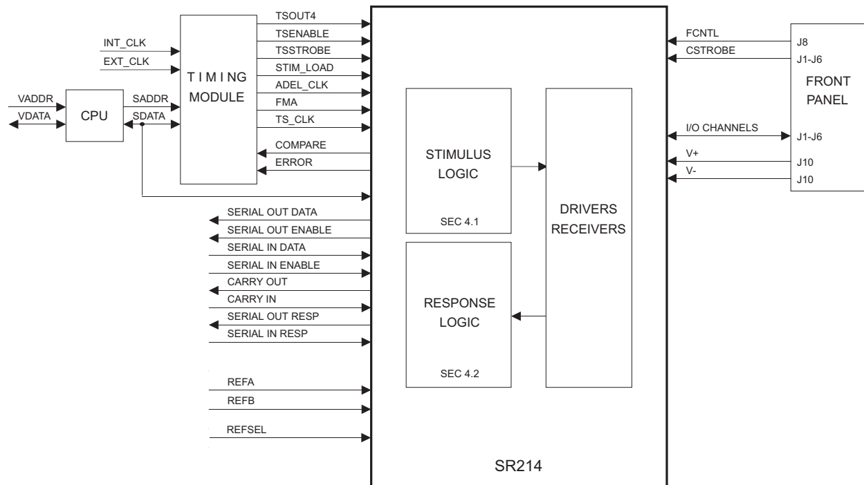
Figure 4-1 SR214 Block Diagram
