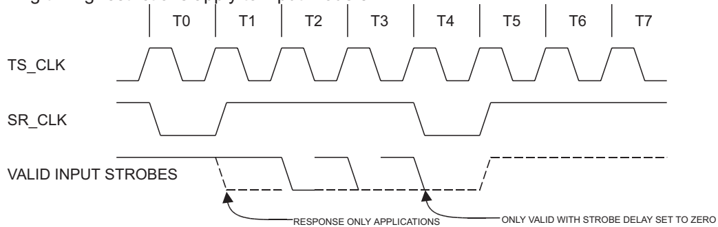
Figure 4-19 Input Mode 3 Timing Restrictions
