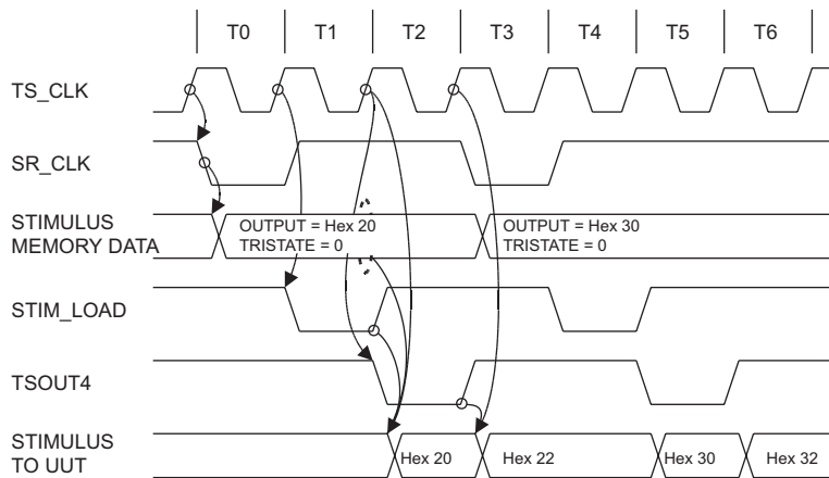
Figure 4-7 INCREMENT2 Timing Example
