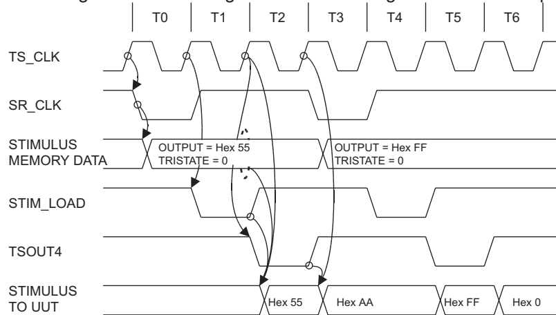
Figure 4-6 RTC Timing Example
