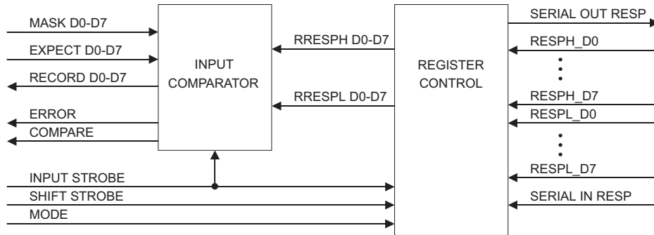
Figure 4-14 Input Mode Logic
