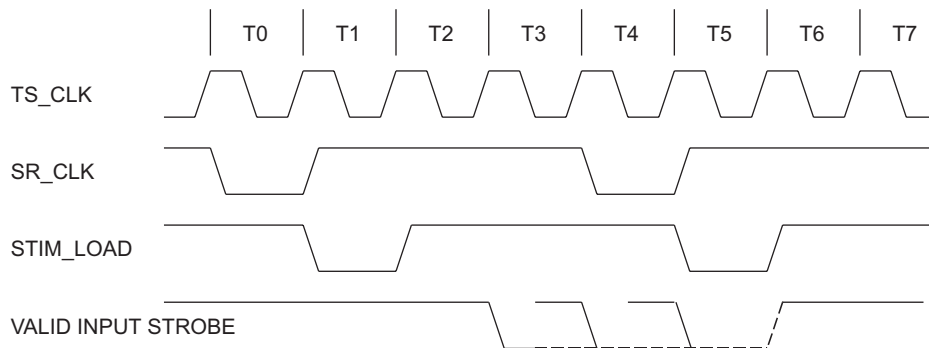
Figure 4-15 Input Mode 1 Timing Restrictions
